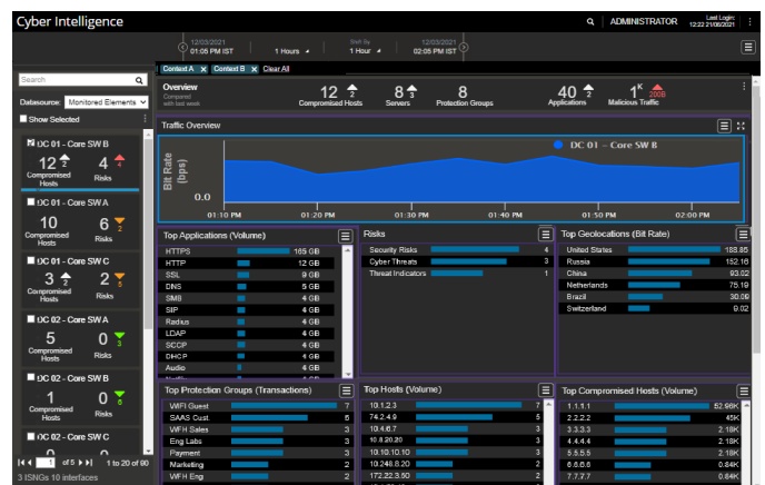
Figure 6: Network Visibility with OCI.
