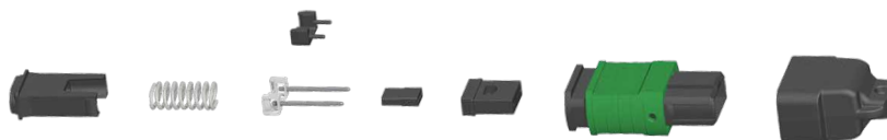
Bare Ribbon without Boot, 20N Spring Force, MTP® Connector (Exploded View)
