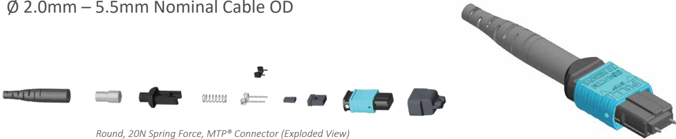
Round, 20N Spring Force, MTP® Connector (Exploded View)
